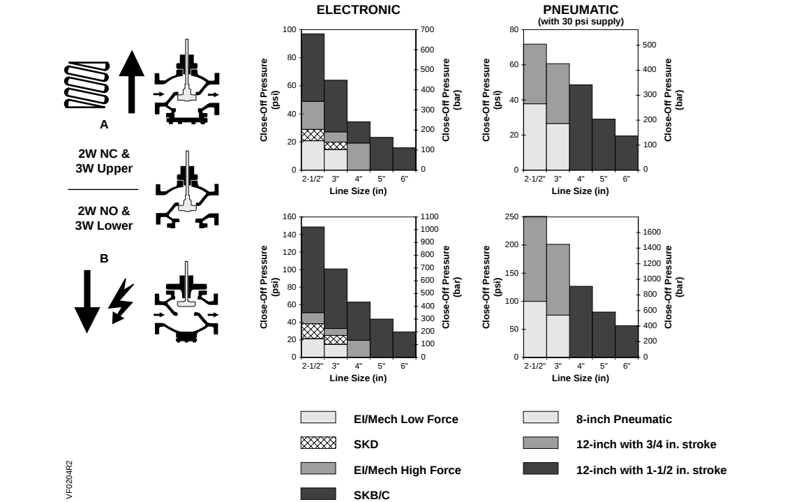
Figure 3. Close-off Pressures for 2-1/2 through 6-Inch Valves.
